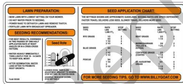
LABEL SEED METERING ITEM #29 P/N 350392 (page 8)
